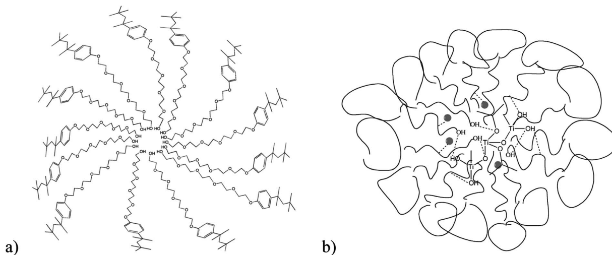
Fig. 10 Schematic illustration of (a) a reversed micelle formed by the Triton X-45 surfactant in a non-polar solvent and (b) the interactions between hydrolysed \text{Ti}(\text{O}i\text{Pr})_4 and the ethylenoxy groups of the polar surfactant tails.
