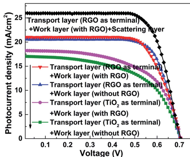
Fig. 4 J-V curves of DSSCs with various photoanodes.
