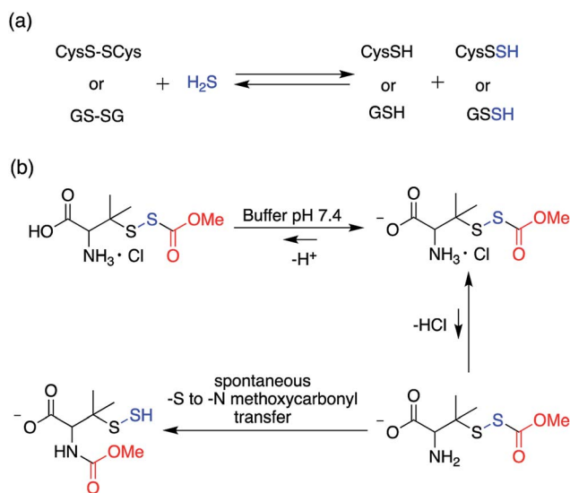
Scheme 4 (a) Generation of small molecule persulfides by reaction of \text{H}_2\text{S} with their corresponding disulfides (b) persulfide analogue of the nitrosothiol S-nitrosoacetylpenicillamine (SNAP).
