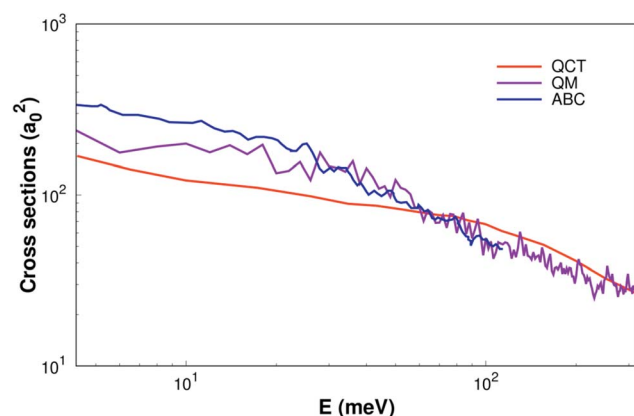
Fig. 6 Integral cross sections of reaction of H(^2S) + CH^+(X^1\Sigma^+) \rightarrow C^+(^2P) + H_2(X^1\Sigma_g^+) as a function of collision energy. The QM and ABC from Li 11 and Schneider 9 are shown as well.
