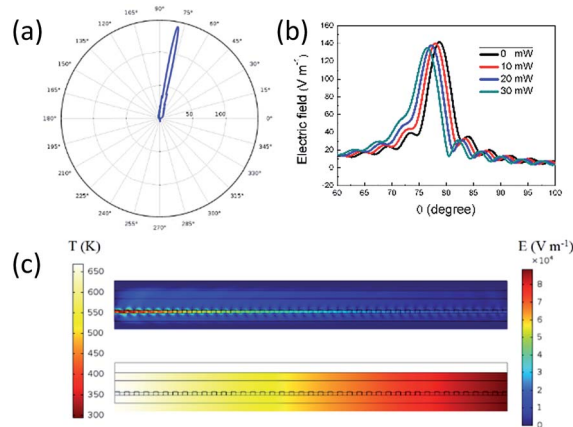
Fig. 13 (a) Polar plot of the far-field radiation pattern. (b) Beam steering for 0\text{--}30\text{ mW} heating power with 10\text{ mW} step. (c) Electric field distribution (upper panel) and thermal field distribution (lower panel) corresponding to 30\text{ mW} .
