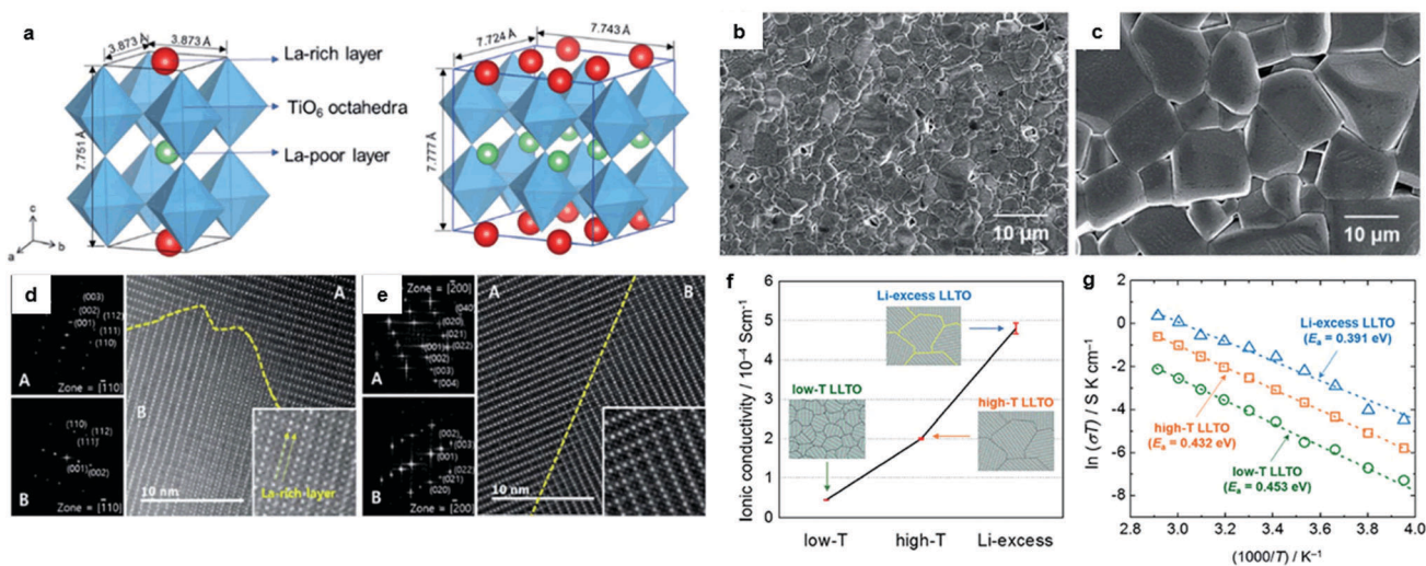
Fig. 2 (a) A schematic of the crystal structures of LLTOs: a tetragonal structure (left) and orthorhombic structure (right). FESEM micrographs of LLTOs sintered at different temperatures; (b) low- T LLTO (1200 °C) and (c) high- T LLTO (1400 °C). HRTEM images combined with SAEDs of (d) low- T LLTO and (e) high- T LLTO (magnified images are given in the inset): (f) a comparison of Li + conductivities along with schematics of the domain microstructures of the LLTO electrolytes: low- T LLTO, high- T LLTO and Li-excess LLTO. (g) Arrhenius plots of the boundary conductivities for low- T LLTO, high- T LLTO and Li-excess LLTO measured over a temperature range of 20 °C to 70 °C. The activation energy ( E_a ) values calculated are indicated. 90 Reproduced with permission from ref. 90. Copyright (2017), the Royal Society of Chemistry.
