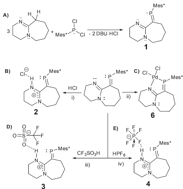
Scheme 2 Simplified synthetic procedures: (A) 1 ; THF, -78^\circ\text{C} (B) 2 ; (i) anhydrous HCl (2 M, THF), THF, -78^\circ\text{C} . (C) 6 ; (ii) [\text{Pd}(\text{MeCN})_2\text{Cl}_2] , DCM, rt. (D) 3 ; (iii) \text{CF}_3\text{SO}_3\text{H} (neat), MS (3 Å), THF, -78^\circ\text{C} . (E) 4 ; (iv) \text{HPF}_6 (60% aq.), MS (3 Å), THF, -78^\circ\text{C} .
