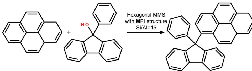
Scheme 2 Alkylation of pyrene with 9-phenyl-9-fluorene-9-ol.
