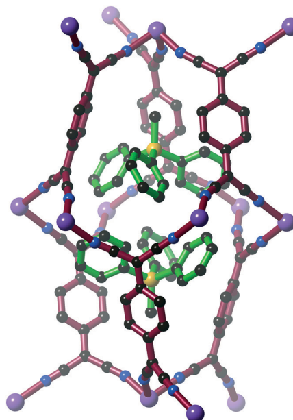
Fig. 12 The structure of (\text{MePPh}_3)_2[\text{M}_2(\text{TCNQ})_3] ( \text{M}^{\text{II}} = \text{Zn, Ni, Co, Fe} ) (65–68) in which there is a significant twist in the TCNQ ^{2-} ligands. Pairs of MePPh _3^+ cations (green) occupy the intra-framework cavities.
