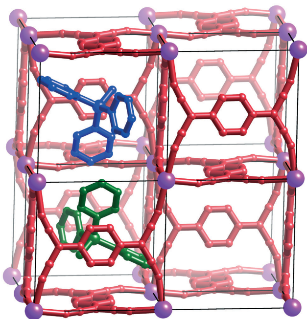
Fig. 11 A representation of (\text{MePPh}_3)_2[\text{Cd}_2(\text{TCNQ})_3] (64) illustrating the pseudo-cubic arrangement of Cd centres. For clarity, only two MePPh _3^+ cations, which occupy "octants" within the framework are shown.
