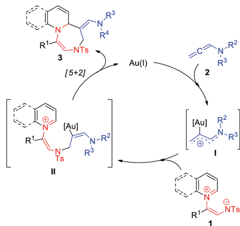
Scheme 2 Plausible mechanism of gold-catalyzed [5+2] cycloaddition.
