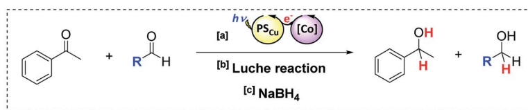
Fig. 3 Conditions: 1 (1 mol%), \text{PS}_{\text{Cu}} (1.5 mol%), total substrate concentration (16.5 mM) in a \text{H}_2\text{O} : \text{CH}_3\text{CN} : ^i\text{Pr}_2\text{EtN} (3 : 2 : 0.1 mL) mixture, irradiated at 447 nm for 3.5 h at 30 °C under \text{N}_2 . The plotted data are the ratio between the amount of the reduced product formed and the sum of the amount of the reduced product formed and the unconverted starting material. The black dotted line indicates where substrates 11d (a), 11f (b), and 11e (c) start reacting.
