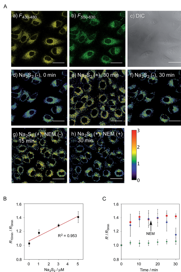
Fig. 4 (A) Fluorescence images of A549 cells treated with 6 -AM (5 \mu\text{M} ). (a) F_{430-480} , (b) F_{550-630} , (c) DIC, and (d) ratio image ( R = F_{430-480}/F_{550-630} ). (e) and (f) Ratio image after 30 min in the presence and absence of \text{Na}_2\text{S}_2 (5 \mu\text{M} ), (g) and (h) ratio image after 15 min in the presence \text{Na}_2\text{S}_2 (5 \mu\text{M} ) and subsequent treatment with NEM (100 \mu\text{M} ) for 15 min. Scale bar: 30 \mu\text{m} . (B) Ratio value change of A549 cells upon the addition of various concentrations of \text{Na}_2\text{S}_2 (0–5 \mu\text{M} ), n = 6. (C) Time trace plot of the ratio value in A549 cells upon the treatment with \text{Na}_2\text{S}_2 (5 \mu\text{M} ) (red square, n = 6), \text{Na}_2\text{S}_2 (5 \mu\text{M} ) and the subsequent addition of NEM (100 \mu\text{M} ) at 15 min (blue circle, n = 4), without \text{Na}_2\text{S}_2 and NEM (green diamond, n = 6).
