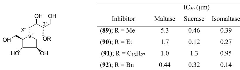
Fig. 25 3'-O-Alkylated analogues (89–92) of salacinol showing different hydrophobic groups and their \text{IC}_{50} ( \mu\text{M} ) values against disaccharidases.
