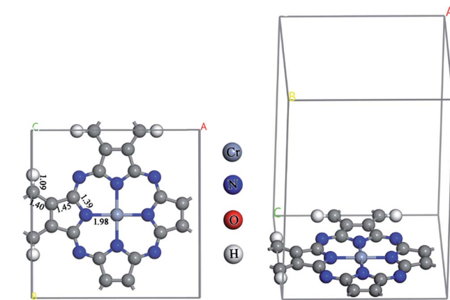
Fig. 1 Top view (left) and side view (right) of the unit cell of CrPc monolayer.
