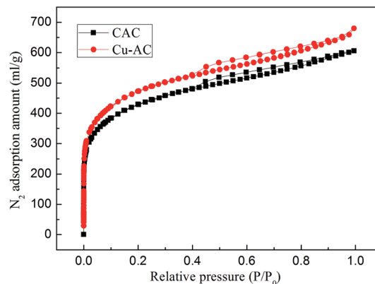
Fig. 2 N 2 adsorption-desorption isotherms of the CAC and Cu-AC.
