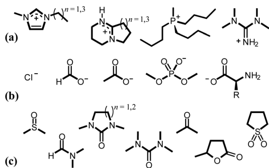
Fig. 4 Typical cations (a), anions (b) and co-solvents (c) incorporated into (IL and) OES solvents for the dissolution of cellulose.
