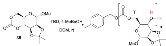
Fig. 27 Organocatalytic ROP of D-mannose derived cyclic carbonate 35 with head–tail regioselectivity.
