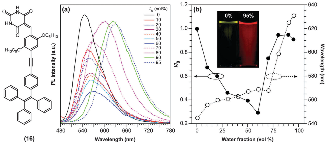
Fig. 7 (a) Emission spectra of 10 mM of the red-emissive barbituric acid-functionalised tetraphenylethene derivative ((16); TPE-HPh-Bar; \lambda_{\text{ex}} = 447 nm) in THF/water mixtures with different water fractions ( f_w ). (b) Plots of relative PL intensities ( I/I_0 ) and emission maxima versus the composition of the THF/water mixture of TPE-HPh-Bar. I_0 = emission intensity in pure THF solution. Inset: Fluorescence emission of TPE-HPh-Bar in THF/water mixtures (0% and 95%) under UV excitation with a portable lamp. Adapted from ref. 60 with permission from the Royal Society of Chemistry ©2014.
