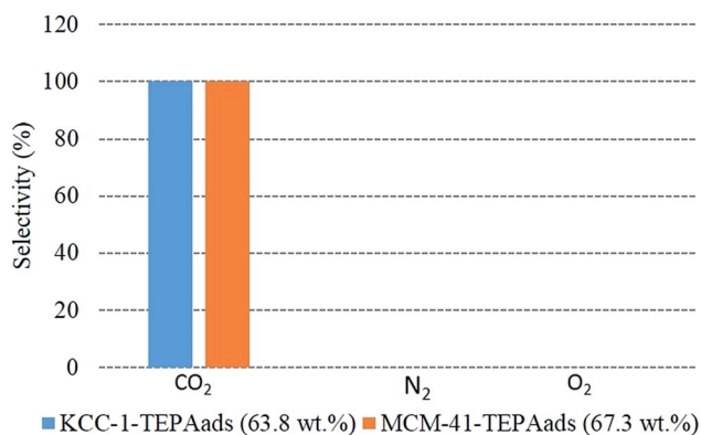
Fig. 11 Sorbent selectivity for CO 2 , N 2 and O 2 at 75 °C.
