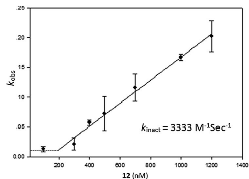
Fig. 3 Plot of the inactivation rate constants ( k obs ) vs. the concentration of 12 (nM), for obtaining the maximal rate of enzyme inactivation ( k inact ). Each value represents the mean ± SE of two independent experiments.
