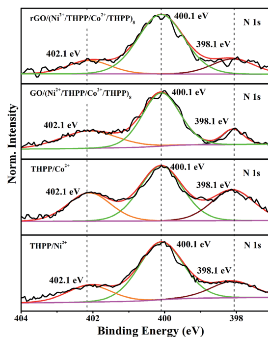
Fig. 2 High-resolution XPS spectra of N 1s of THPP/ \text{Ni}^{2+} , THPP/ \text{Co}^{2+} , \text{GO}/(\text{Ni}^{2+}/\text{THPP}/\text{Co}^{2+}/\text{THPP})_8 and \text{rGO}/(\text{Ni}^{2+}/\text{THPP}/\text{Co}^{2+}/\text{THPP})_8 .
