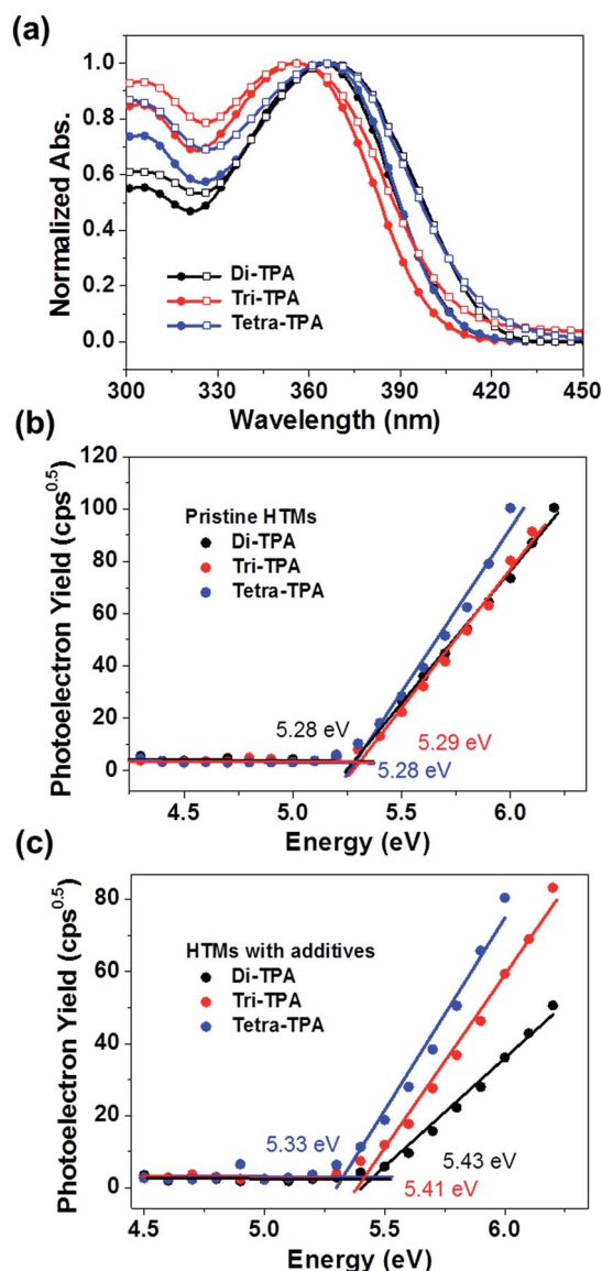
Fig. 2 (a) UV-vis spectra of HTMs in toluene (●) and film (□). (b and c) PES data of HTMs with and without additives; the lines are linear fits of the data.
