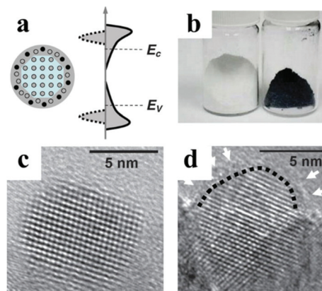
Fig. 10 (a) Scheme of the structure and band gap of \text{TiO}_2 black; (b) photographs of \text{TiO}_2 white (left) and \text{TiO}_2 black (right) samples; High Resolution Transmission Electron Microscopy (HRTEM) images of (c) anatase NCs and (d) \text{TiO}_2 black (modified with permission from ref. 104, copyright 2011 American Association for the Advancement of Science).
