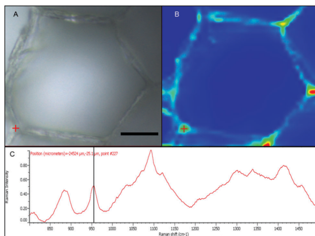
Fig. 6 Macrocystis cortex. (A) Brightfield. (B) Heatmap of the 955\text{ cm}^{-1} Raman shift. (C) Raman spectrum of the point indicated by the red crosshairs in (A) and (B). Scalebar, 20 μm.
