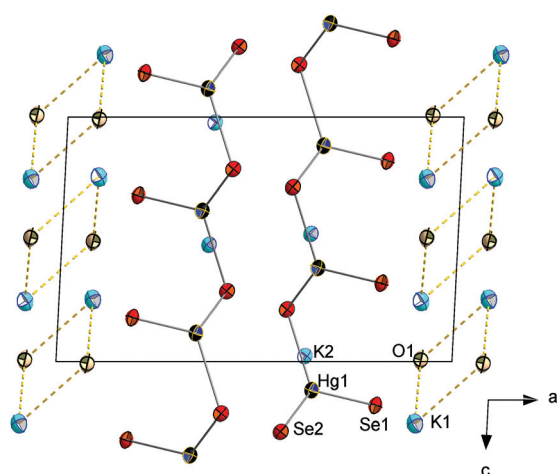
Fig. 4 Fragment of the crystal structure of 4. Ellipsoids are drawn at 50% probability. Selected structural parameters [ \text{\AA} , ^\circ ]: Hg–Se1: 2.5097(10), Hg–Se2: 2.5908(10)–2.6090(11), K...Se: 3.193(2)–3.497(2), K...O: 2.789(9)–3.426(9), Se–Hg–Se: 107.19(3)–132.38(3).
