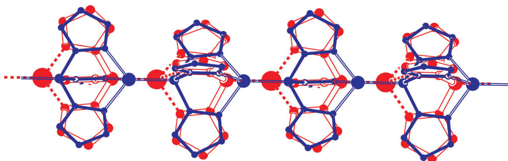
Fig. 8 Disorder in the one-dimensional Cu coordination chain of [(\text{H}^+\text{Cu})[\text{PF}_6])_n . Location in the unit cell at (2/3, 1/3, z) , Wyckoff position b . The major disorder component is drawn in red, the minor component in blue. The estimated ratio between the two components is 65 : 35%.
