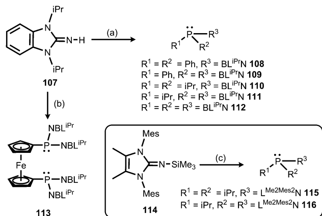
Scheme 25 Synthesis of benzimidazolin-2-imino-substituted phosphines 108 – 113 , as well as the imidazolin-2-imino-substituted phosphines 115 and 116 . (a) (1) n BuLi, THF, -78^\circ\text{C} ; (2) chlorophosphine, room temperature. (b) (1) n BuLi, THF, -78^\circ\text{C} ; (2) [\text{Fe}(\text{C}_5\text{H}_4\text{PCl}_2)_2] . (c) 115 : \text{iPr}_2\text{PCL} , THF; 116 : (1) \text{PCl}_3 , THF, -78^\circ\text{C} ; (2) \text{iPrMgCl} , THF, -78^\circ\text{C} .
