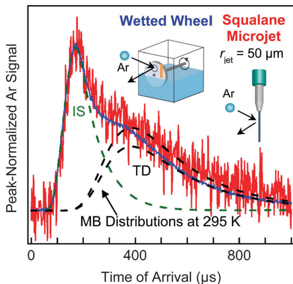
Fig. 7 TOF spectra following collisions of 90 \text{ kJ mol}^{-1} Ar atoms with a squalane flat film (blue) and a 50 \text{ }\mu\text{m} radius microjet (red). The black dashed lines are Maxwell-Boltzmann distributions at T_{\text{liq}} = 295 \text{ K} , and the green dashed line shows the inelastic scattering (IS) component. Spectra have been peak-normalized for comparison. Adapted with permission from D. K. Lancaster, A. M. Johnson, D. K. Burden, J. P. Wiens and G. M. Nathanson, J. Phys. Chem. Lett. , 2013, 4 , 3045–3049. Copyright 2013 American Chemical Society.
