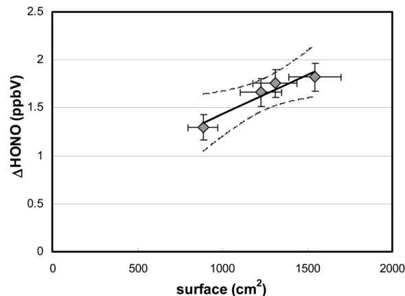
Fig. 4 HONO formation in the photolysis of adsorbed HNO 3 as a function of the reactor surface area ( [\text{HNO}_3]_{\text{surf}} = 1.6 \times 10^{14} \text{ cm}^{-2} , [\text{HNO}_3]_{\text{g}} = 86 \text{ ppbV} , 59% r.h.). The straight line represents the linear regression of the data ( r^2: 0.93 ) with its 95% confidence limits (dashed lines).
