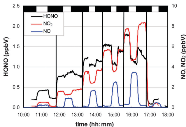
Fig. 3 HONO and NO x formation from photolysis of adsorbed HNO 3 ( 7.8 \times 10^{13} \text{ cm}^{-2} ) in the flow-reactor continuously flushed with humid (54% r.h.) gas-phase HNO 3 . After first irradiation, NO 2 was added stepwise to the HNO 3 mixture (marked with vertical black lines). For the last step, the NO 2 addition was set to zero again. The vertical bars above the plot represent dark (black) and irradiated (white) periods.
