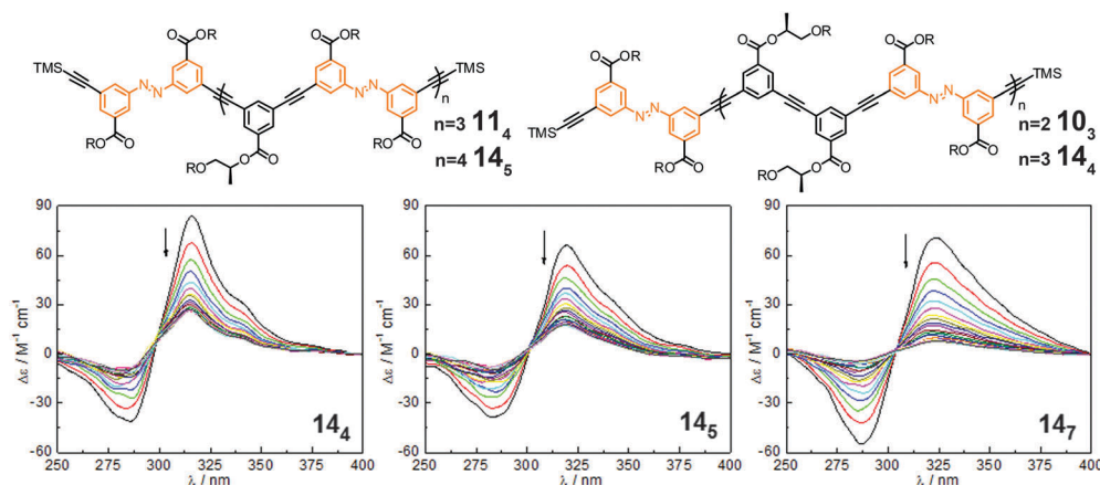
Fig. 15 Photoswitchable oligoazobenzene tetradecamers 14 4 , 14 5 , and 14 7 ( R = -(CH_2CH_2O)_3CH_3 ) and their corresponding CD spectra during the course of irradiation at \lambda_{irr} = 358 nm in CH_3CN at 25 °C. 106
