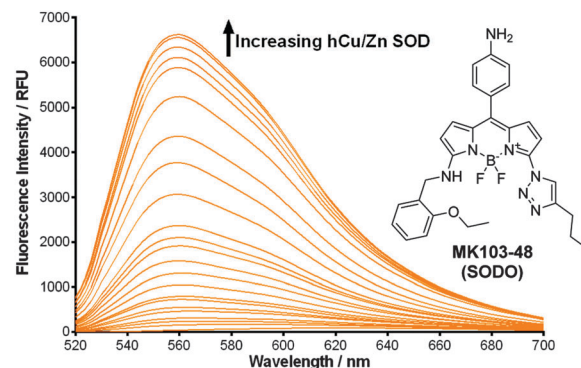
Fig. 1 Chemical structure and fluorescence spectra of SODO ( 10 \mu\text{M} ) after incubation with serial concentrations of hCu/Zn-SOD from 0.01 to 5 \text{ mg mL}^{-1} in 20 mM Tris-HCl buffer (pH = 7.4). \lambda_{\text{exc}} : 460 nm. \Phi_F in hCu/Zn-SOD: 0.45.
