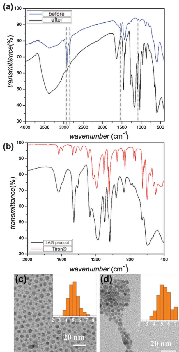
Fig. 1 Comparison of FTIR-ATR spectra for: (a) precursor IONPs 1 before (blue) and after (black) LAG with Tiron (100 mg Tiron, 10 \mu\text{L} toluene), demonstrating the almost complete disappearance of characteristic oleic acid absorption bands namely \text{CH}_2 stretches at 2800\text{--}3000 \text{ cm}^{-1} and \text{COO}^- stretches at 1520 \text{ cm}^{-1} and 1448 \text{ cm}^{-1} . Dashed lines are guides for the eye; (b) Tiron reactant and product of LAG of 1 and Tiron (100 mg Tiron, 10 \mu\text{L} toluene). Spectra in (a) and (b) confirm the mechanochemical replacement of surface oleic acid on 1 with Tiron. Comparison of TEM images for 1 : (c) before and (d) after LAG with Tiron, demonstrating the retention of nanoparticle size and low size dispersity. Insets show size distribution (see also ESI,† Fig. S5).
