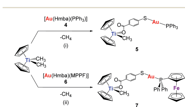
Scheme 1 Preparation of heterometallic titanocene-gold complexes [(\eta\text{-C}_5\text{H}_5)_2\text{Ti}(\text{CH}_3)(\text{OC}(\text{O})\text{C}_6\text{H}_4\text{SAu}(\text{PR}_2\text{R}'))] ( \text{R} = \text{R}' = \text{Ph} , 5 ; \text{R} = \text{Ph} , \text{R}' = \text{ferrocene} , 7 ). (i) THF/toluene 1.5 : 1, RT, 1 h; (ii) acetonitrile/toluene 3 : 1, RT, 1 h.
