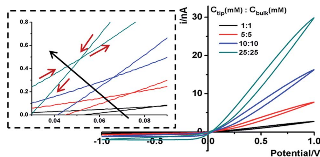
Fig. 2 Representative I-V features of a 60 nm radius nanopipette in symmetric tip–bulk KCl concentrations. The scan rate is 100 mV s −1 . The inset shows the scan directions and the cross-point positions of all I-V curves. The shift in cross-point with the increase of concentration is indicated by the long arrow.
