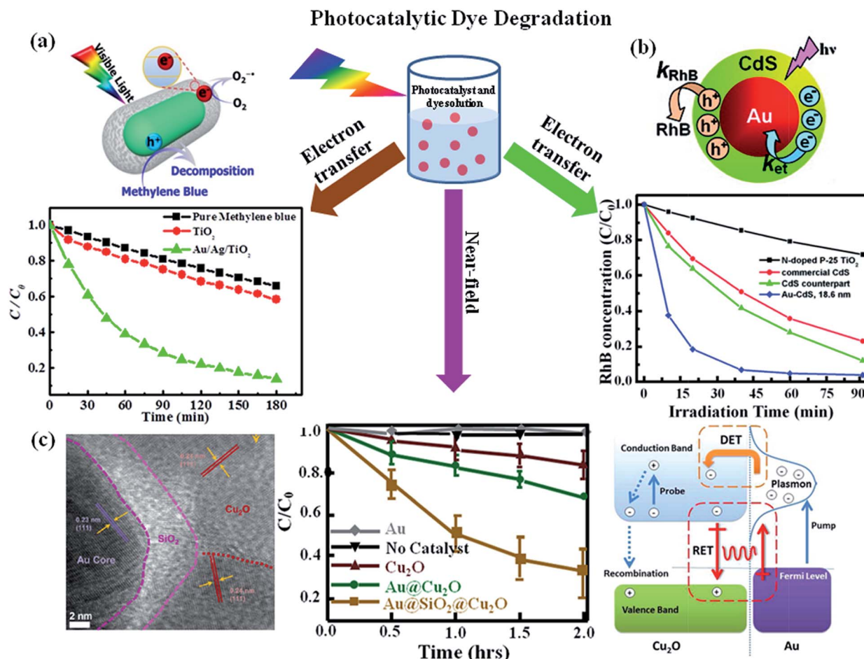
Fig. 9 Photocatalytic dye degradation: (a) photocatalytic degradation of MB under visible light irradiation in the absence and presence of photocatalysts (P25- \text{TiO}_2 , \text{Au@TiO}_2 or \text{Au/Ag/TiO}_2 core-shell NPs) and the schematic representation for the mechanism of photocatalytic degradation of dyes upon visible light excitation of \text{Au/TiO}_2 NRs. (b) Photocatalytic degradation of RhB in the presence of \text{Au/CdS} , CdS and P25- \text{TiO}_2 . The data shows that \text{Au/CdS} NPs exhibit higher catalytic activity and the proposed mechanism to explain the plasmonic metal enhancement is shown in schematic representation. (c) TEM image of \text{Au/SiO}_2/\text{Cu}_2\text{O} NP section, visible-light photodegradation of methyl orange versus time monitored without catalyst and with catalysts Au, \text{Cu}_2\text{O} control, \text{Au/Cu}_2\text{O} , and \text{Au/SiO}_2/\text{Cu}_2\text{O} nanostructures and the schematic representation of various transfer mechanisms for the enhanced catalytic activity of \text{Au/Cu}_2\text{O} nanostructure. Figures (a), (b) and (c) reproduced with permission from ref. 32, 92, and 57, respectively.
