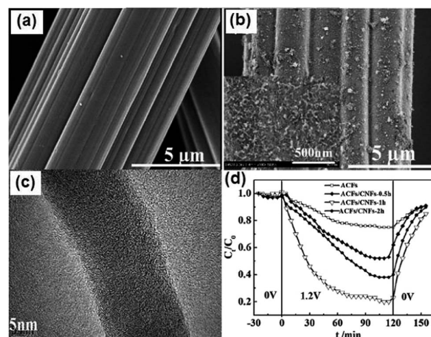
Fig. 13 SEM images of (a) ACFs and (b) ACFs/CNFs-1 h; (c) TEM image of ACFs/CNFs-1 h; (d) electrosorption process for the different electrodes in NaCl solution. Initial 30 \text{ min} : physical absorption; subsequent 120 \text{ min} : electrosorption; final 30 \text{ min} : desorption. The inset in (b) is the corresponding magnified image. (Reproduced with permission from ref. 102.)
