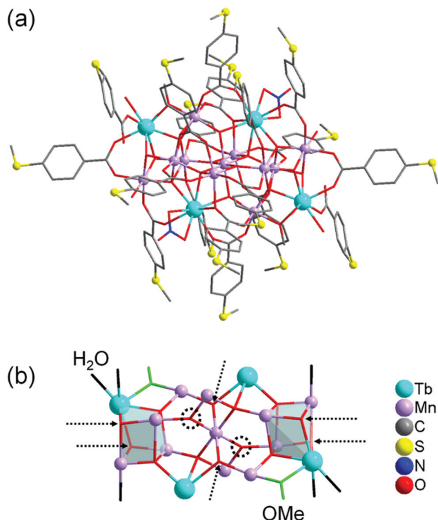
Fig. 1 (a) Molecular structure of compound 1 . (b) Metal–oxide skeleton \{\text{Mn}_{11}\text{Tb}_4\text{O}_{14}\} of compound 1 incorporating two methoxide anions and six water molecules (eighteen bza-SMe − ligands and two NO 3 − ligands are not shown). Six possible \mu_3 -O protonation sites are indicated by dashed arrows and the two remaining, nonprotonated \mu_3 -oxygen atoms by dashed circles. Hydrogen atoms are omitted for clarity. The metal and sulfur atoms are represented as ball-and-stick models. Selected bond lengths [Å]: Tb–O (of H 2 O) 2.371(10) and 2.427(9), Tb–O (of MeO − ) 2.282(8), Tb– \mu_3 -O 2.366(8)–2.492(8), Tb– \mu_4 -O 2.388(7)–2.565(7), Mn–O (of H 2 O) 2.212(9), Mn–O (of MeO − ) 1.891(8), Mn– \mu_3 -O 1.870(7)–2.300(8), Mn– \mu_4 -O 1.860(7)–2.440(7), nearest-neighbor Mn–Tb 3.4045(18), nearest-neighbor Mn–Mn 2.855(2). All bond lengths and angles are reported in the ESI†
