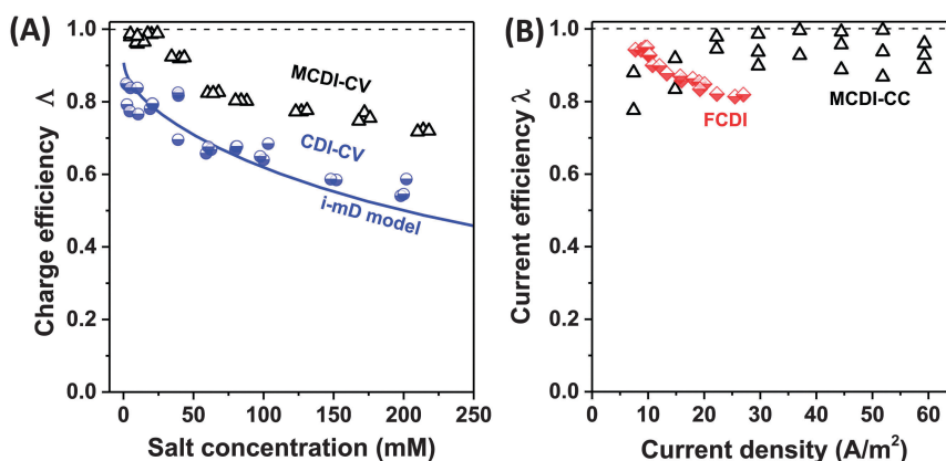
Fig. 6 Selected data for charge efficiency \Delta and current efficiency \lambda as function the salt concentration (A) and current density (B). Data for charge efficiency (A) are obtained for solid film electrodes at V_{\text{ch}} = 1.2 V in a cycle where V_{\text{disch}} = 0 V. Solid line denotes calculation results based on the improved mD model, see ref. 7. The data for current efficiency (B) is obtained for constant-current MCDI (open triangles; ref. 26), and for FCDI (half-filled diamonds; ref. 44).
