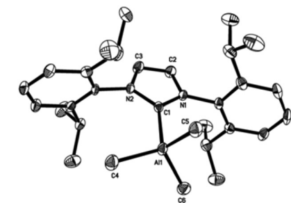
Fig. 5 Molecular structure of IPr-AlMe 3 (3). Thermal ellipsoids are drawn at the 50% probability level. Hydrogen atoms were omitted for clarity. Selected bond lengths [Å] and angles [°] for 3: Al(1)–C(1) 2.103(3), Al(1)–C(4) 1.992(3), Al(1)–C(5) 1.994(3), Al(1)–C(6) 1.994(3), C(1)–N(1) 1.370(4), C(1)–N(2) 1.370(4), C(2)–N(1) 1.387(4), C(3)–N(2) 1.385(4), C(2)–C(3) 1.351(4), C(4)–Al(1)–C(5) 111.5(1), C(4)–Al(1)–C(1) 109.6(1), C(4)–Al(1)–C(6) 111.3(1), C(5)–Al(1)–C(6) 113.6(1), C(5)–Al(1)–C(1) 104.7(1), C(6)–Al(1)–C(1) 105.7(1), N(1)–C(1)–N(2) 103.1(2).
