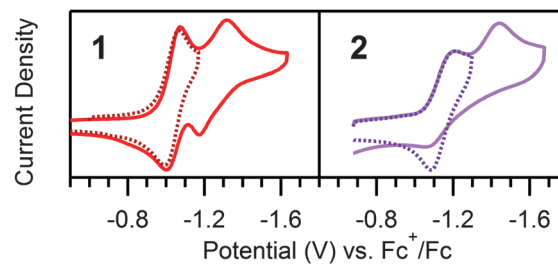
Fig. 2 Cyclic voltammograms of 0.20 mM 1 and 2 without acid at 100 \text{mV s}^{-1} and with 0.1 M [\text{Bu}_4\text{N}][\text{PF}_6] . The \text{Ni}^{\text{II}}/\text{Ni}^{\text{I}} reduction of 1 is reversible (dotted trace) and the \text{Ni}^{\text{I}}/\text{Ni}^0 reduction is quasi reversible. The \text{Ni}^{\text{II}}/\text{Ni}^{\text{I}} reduction of 2 is reversible (dotted trace); however the \text{Ni}^{\text{I}}/\text{Ni}^0 reduction is irreversible.
