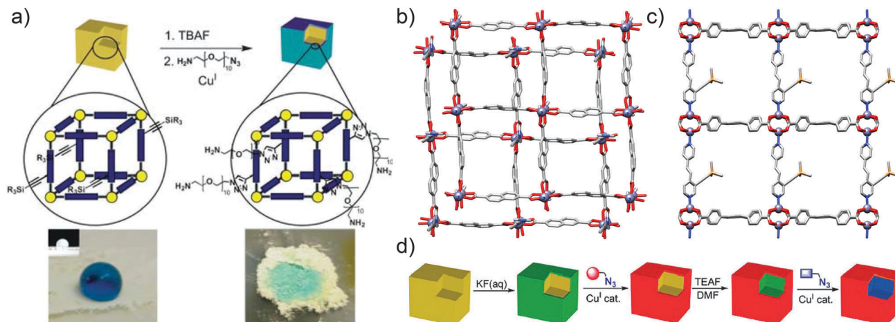
Fig. 16 (a) Selective surface deprotection of alkyne units of [Zn_2(2,6\text{-ndc})_2(\text{TMS-alkyne-1,2-bpe})]_n allows surface modification with hydrophilic PEG groups, significantly changing the wettability of the MOF. Reproduced from ref. 60 with permission from The Royal Society of Chemistry. (b) Crystal structure of the underlying [Zn_2(2,6\text{-ndc})_2(1,2\text{-bpe})]_n framework, redrawn from CCDC deposition PITREQ. (c) Crystal structure of the TMS-alkyne substituted [Zn_2(1,2,4,5\text{-tcbp})(\text{TMS-alkyne-1,2-bpe})]_n , redrawn from CCDC deposition LURGEL, which can (d) be surface modified through selective deprotection of the alkyne groups, and subsequently functionalised throughout the remainder of the material to produce a core-shell functionalised species. Reprinted (adapted) with permission from ref. 61. Copyright (2009) American Chemical Society.
