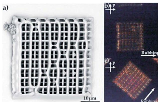
Fig. 5 Left: a 4-layer woodpile structure with 5 μm line distance and 1.3 μm distance between two consecutive layers. The structure is obtained by direct laser writing of azobenzene-containing LC elastomers. Right: polarized-optical micrographs of the LC elastomer woodpiles at different angles of the LC alignment direction with respect to the analyzer. Reproduced with permission from ref. 86. Copyright 2014, Wiley-VCH.
