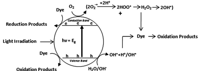
Fig. 2 Pictorial representation of indirect dye degradation process. 24
