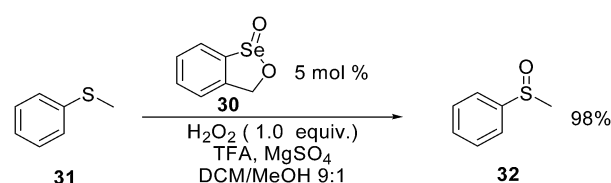
Scheme 27 Oxidation of sulfides to sulfoxides.
