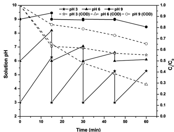
Fig. 4 Effect of solution pH on residual pH changes and COD removal kinetics of the PC-pH process at an applied voltage of 7 V.
