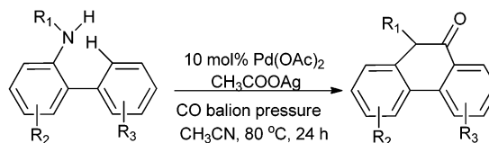
Scheme 17 Reagents and conditions: N-sulfonyl-2-aminobiaryl (50.0 mg), Pd(OAc) 2 (10 mol%), CH 3 COOAg (5 equiv.), 4 mL of anhydrous CH 3 CN, CO balloon, temp. 80 °C, time 24 h.
