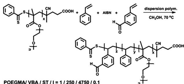
Scheme 1 Synthesis of block copolymers via in situ self-assembly in methanol.
