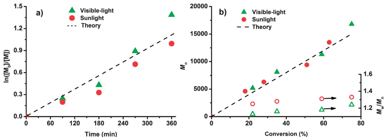
Fig. 4 Visible light- or sunlight-induced ATRP of methyl methacrylate ( [\text{MMA}]_0/[\text{EtBP}]_0/[\text{Cu}^{\text{II}}\text{Br}_2]_0/[\text{PMDETA}]_0/[\text{Mn}_2(\text{CO})_{10}]_0 = 200/1/0.2/0.2/0.05 ): (a) kinetic plot and (b) molecular weights and distributions of the resulting polymers as a function of degree of conversion.
