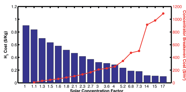
Fig. 6 The bar graph shows the base hydrogen production cost (excluding the cost for solar concentration) as a function of light concentration. The red line shows the break-even cost for the economically viable implementation of a solar-concentrator and tracking components. (Results are based on a multi-junction thin-film Si PV cell).
