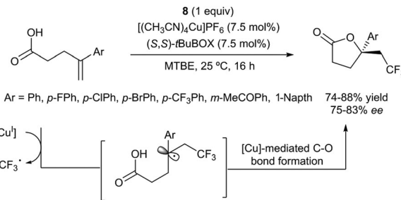
Scheme 22 Copper-catalyzed enantioselective oxotrifluoromethylation of unactivated olefins.
